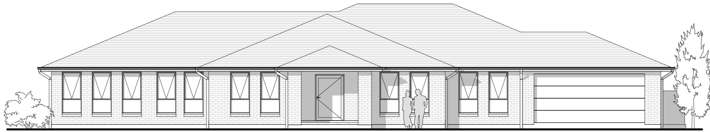
FRONT ELEVATION 1:100
