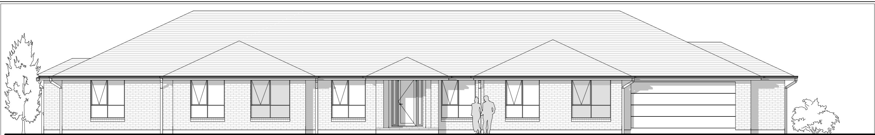
FRONT ELEVATION 1:100
