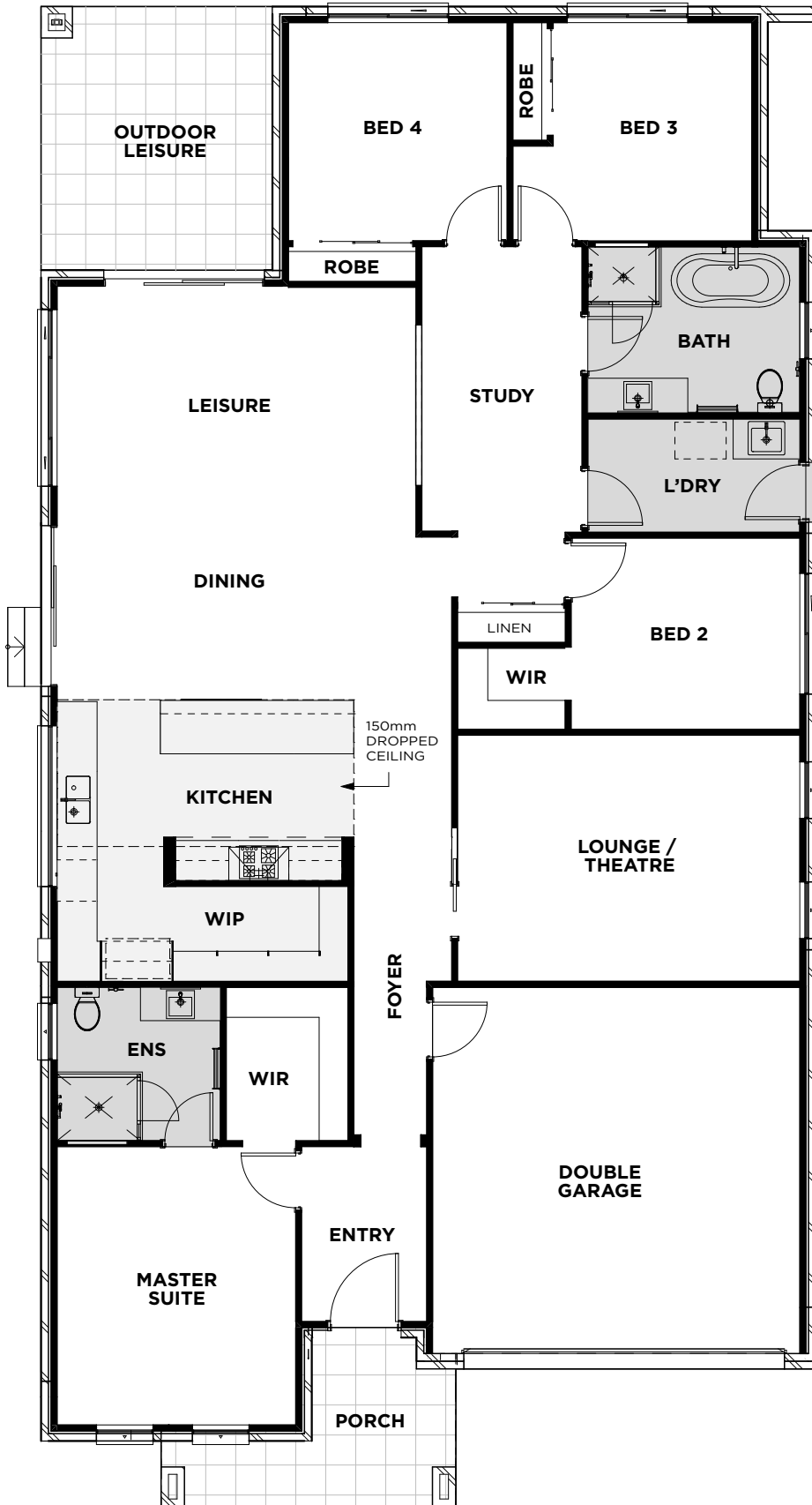
GROUND FLOOR
