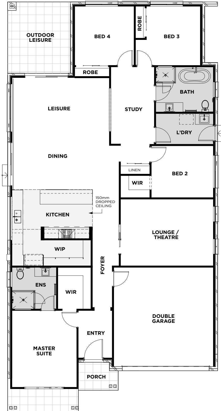
GROUND FLOOR
