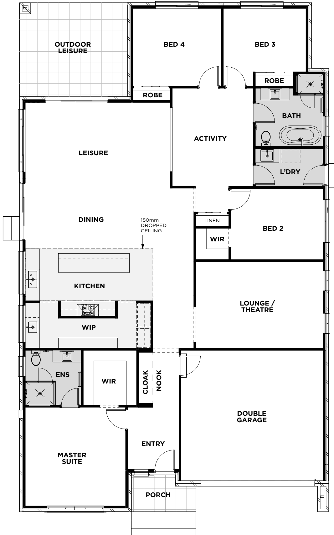
GROUND FLOOR
