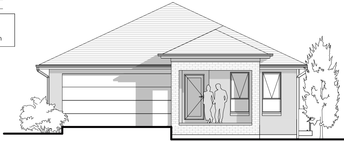
FRONT ELEVATION 1:100
