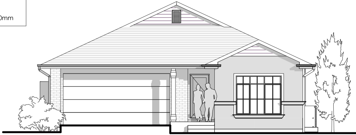
FRONT ELEVATION 1:100
