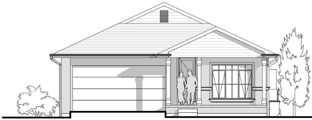
FRONT ELEVATION 1:100
