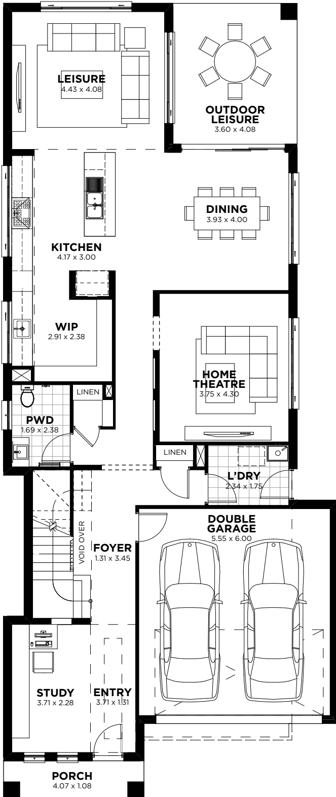
GROUND FLOOR
