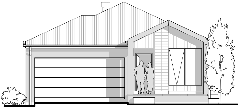
FRONT ELEVATION1:100
