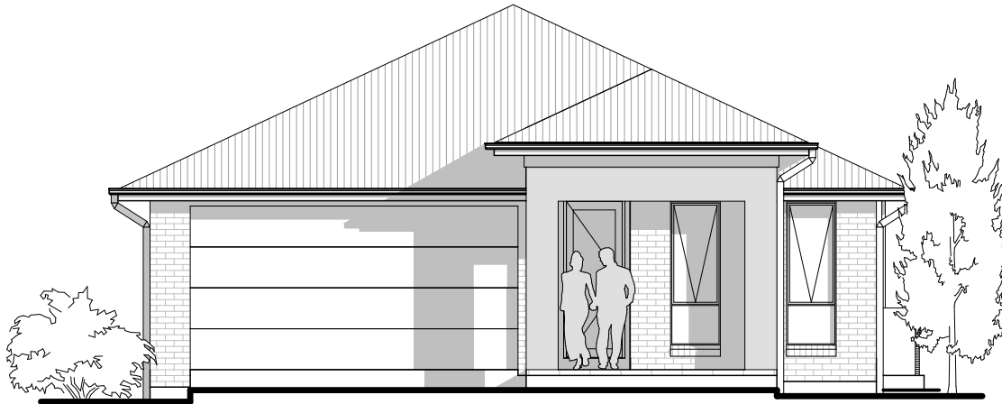
FRONT ELEVATION 1:100
