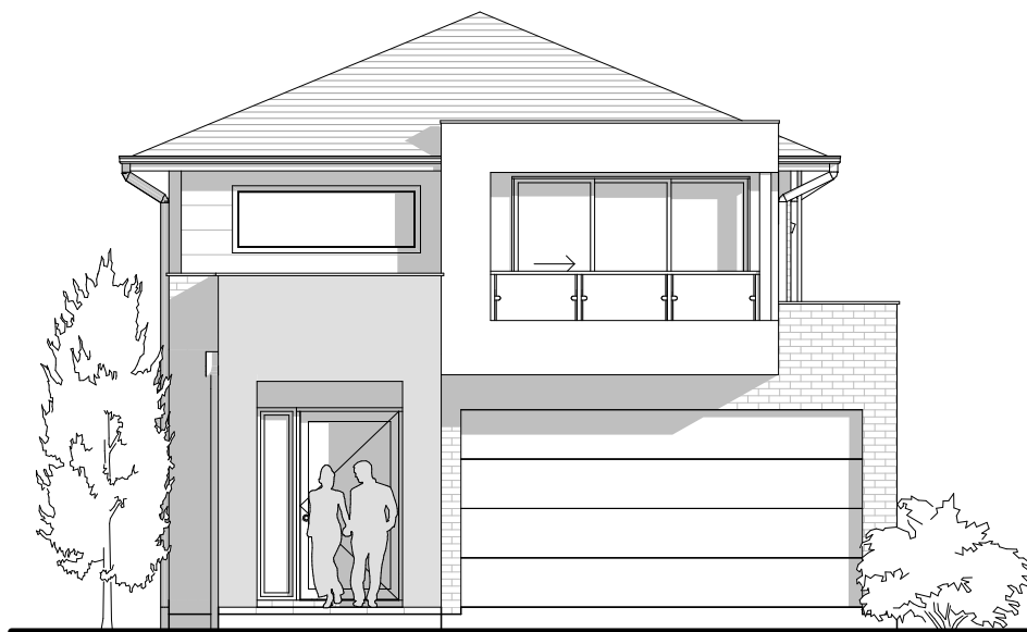
FRONT ELEVATION 1:100
