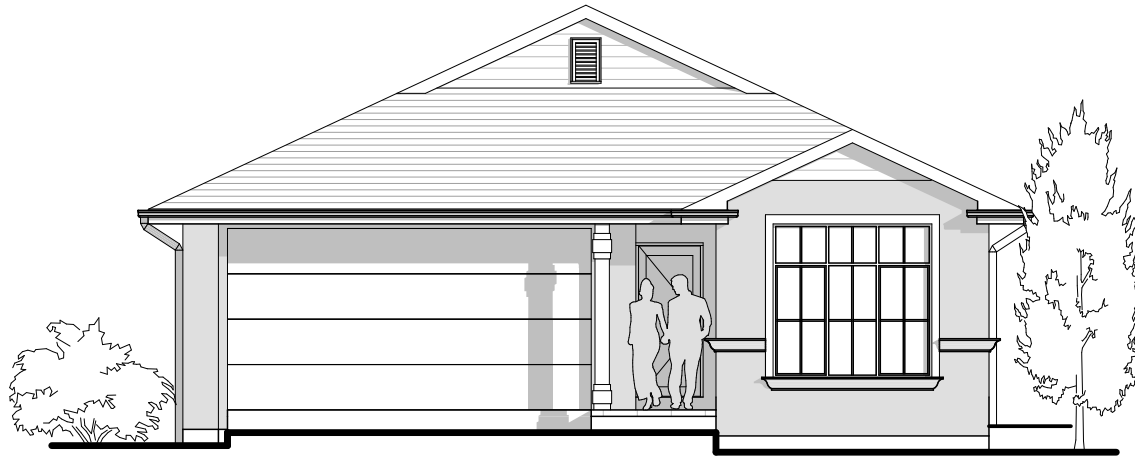
FRONT ELEVATION 1:100
